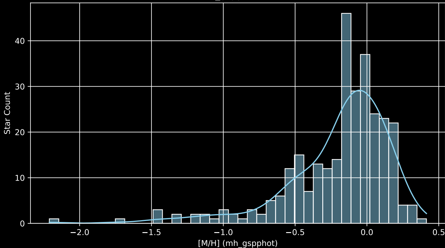
APOGEE DR17 Field: [345-12 [M/H] (mh_gspphot) (n= 297)
