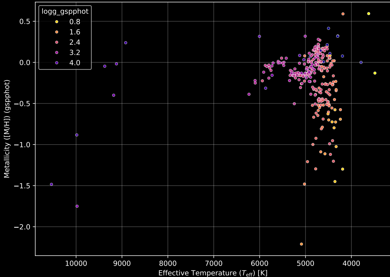
APOGEE DR17 Field: [345-12] Stellar Population Parameters (n= 299)
