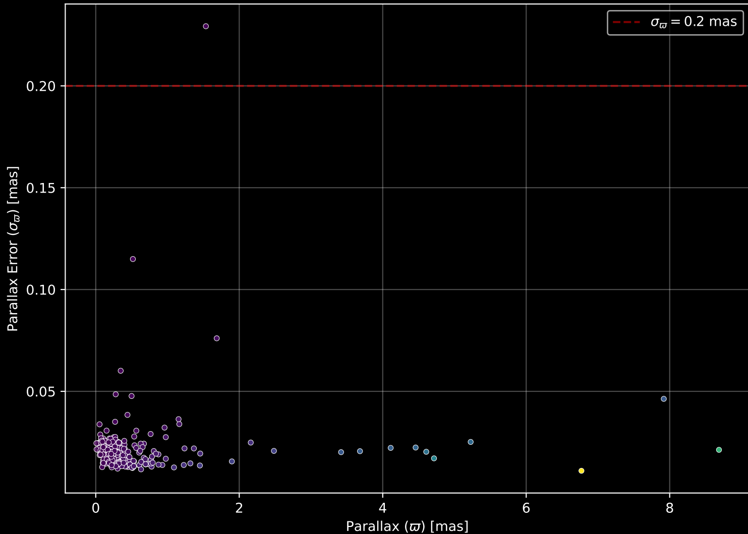
APOGEE DR17 Field: [345-12] Parallax Quality (n= 299)
