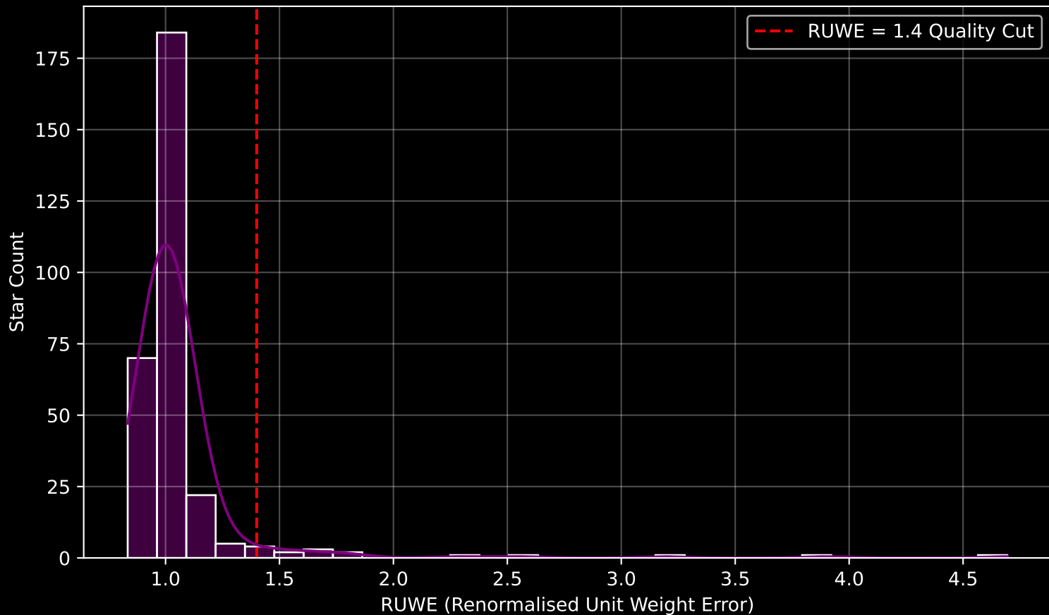
GAPOGEE DR17 Field [345-12] RUWE Distribution (n= 297)
