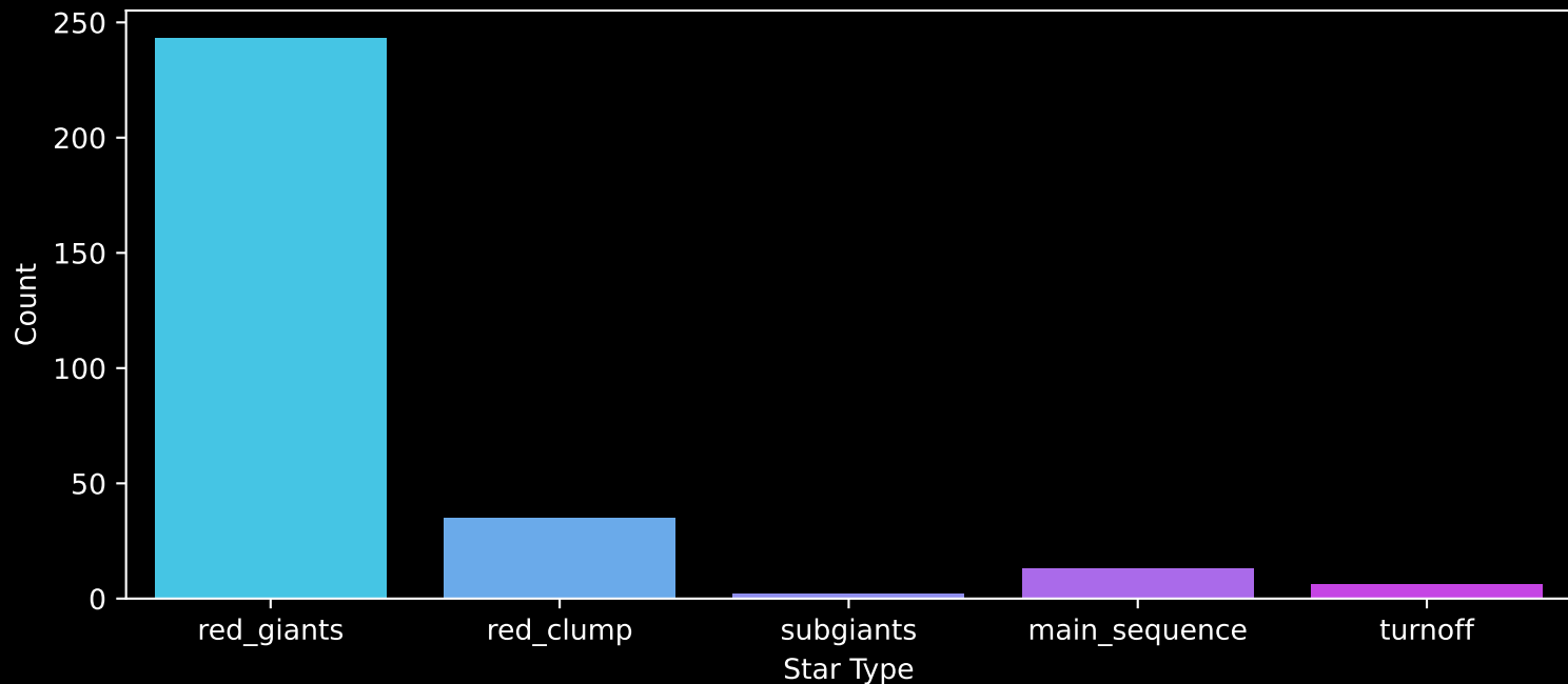
APOGEE DR17 Field: [345-12] Count plot of Star Type
