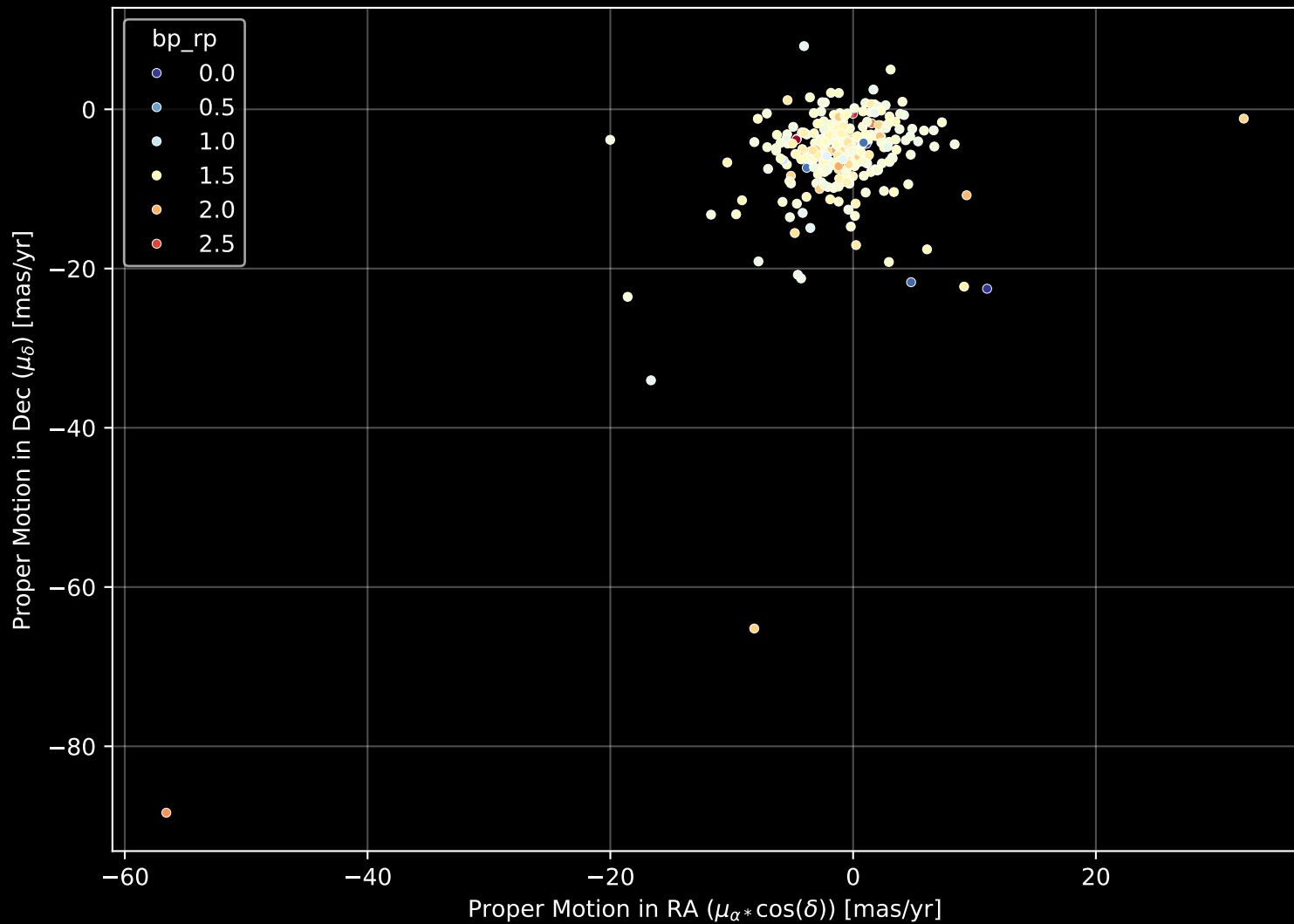
APOGEE DR17 Field: [345-12] Proper Motion Diagram (n= 299)
